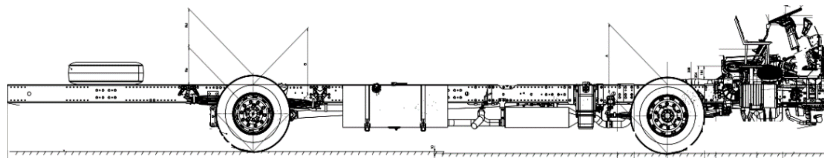
Chassis height
