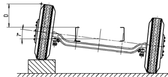
Front axle
