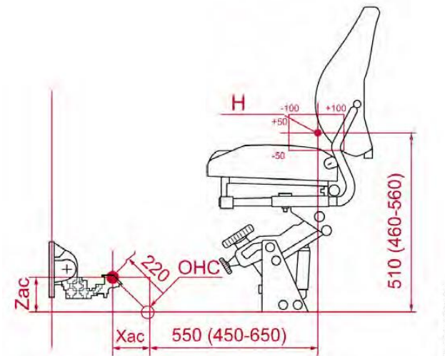
Driver's seat Ergonomics
