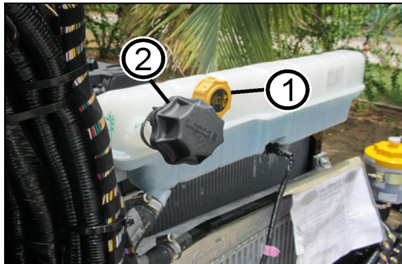
Expansion tank 1 Pressure valve 2 Filler neck
