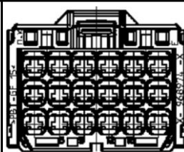
Bus Body Interconnector
